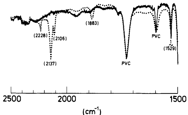
Figure 3. Irradiation ( \lambda 370 nm) of diphenylnitrilimine (2) in PVC at 85 K with formation of benzonitrile ( \nu_{\max} 2228 \text{cm}^{-1} ), diphenylcarbodiimide ( \nu_{\max} 2137, 2106 \text{cm}^{-1} ), and 1-aza-1,2,4,6-cycloheptatetraene (6) ( \nu_{\max} 1883 \text{cm}^{-1} ) monitored by IR spectroscopy.
